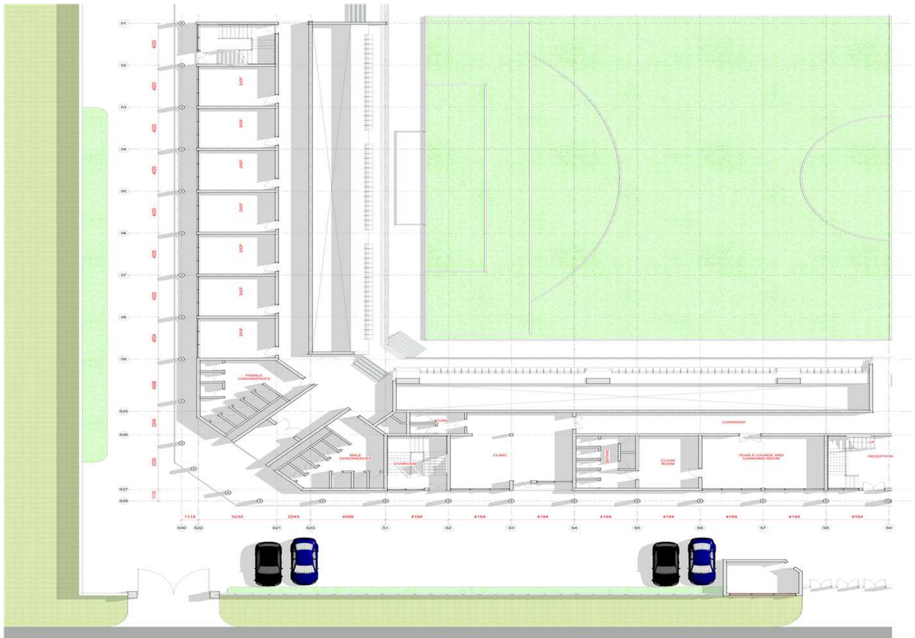
03a- GROUND FLOOR PLAN
