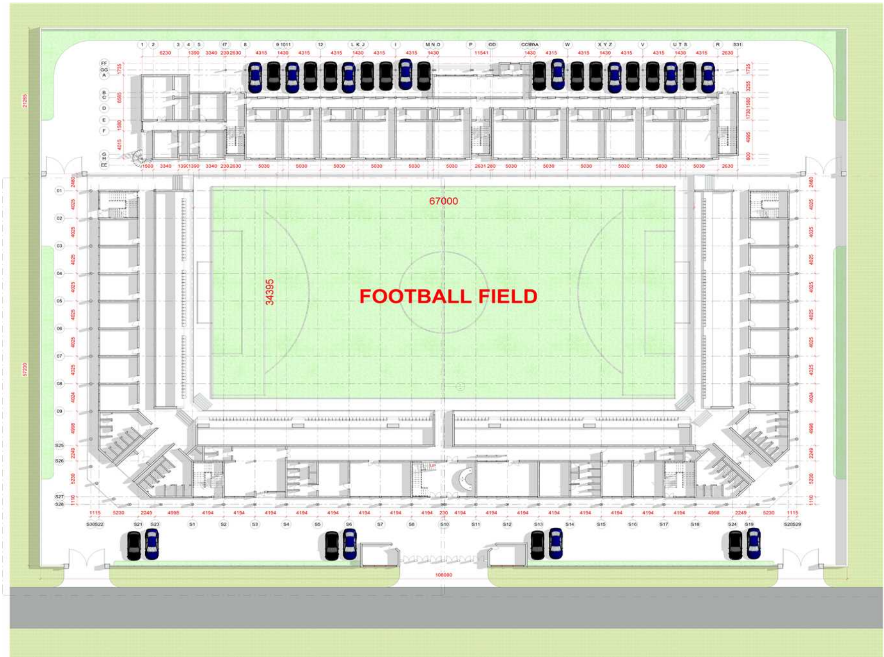
01- GROUND FLOOR PLAN
