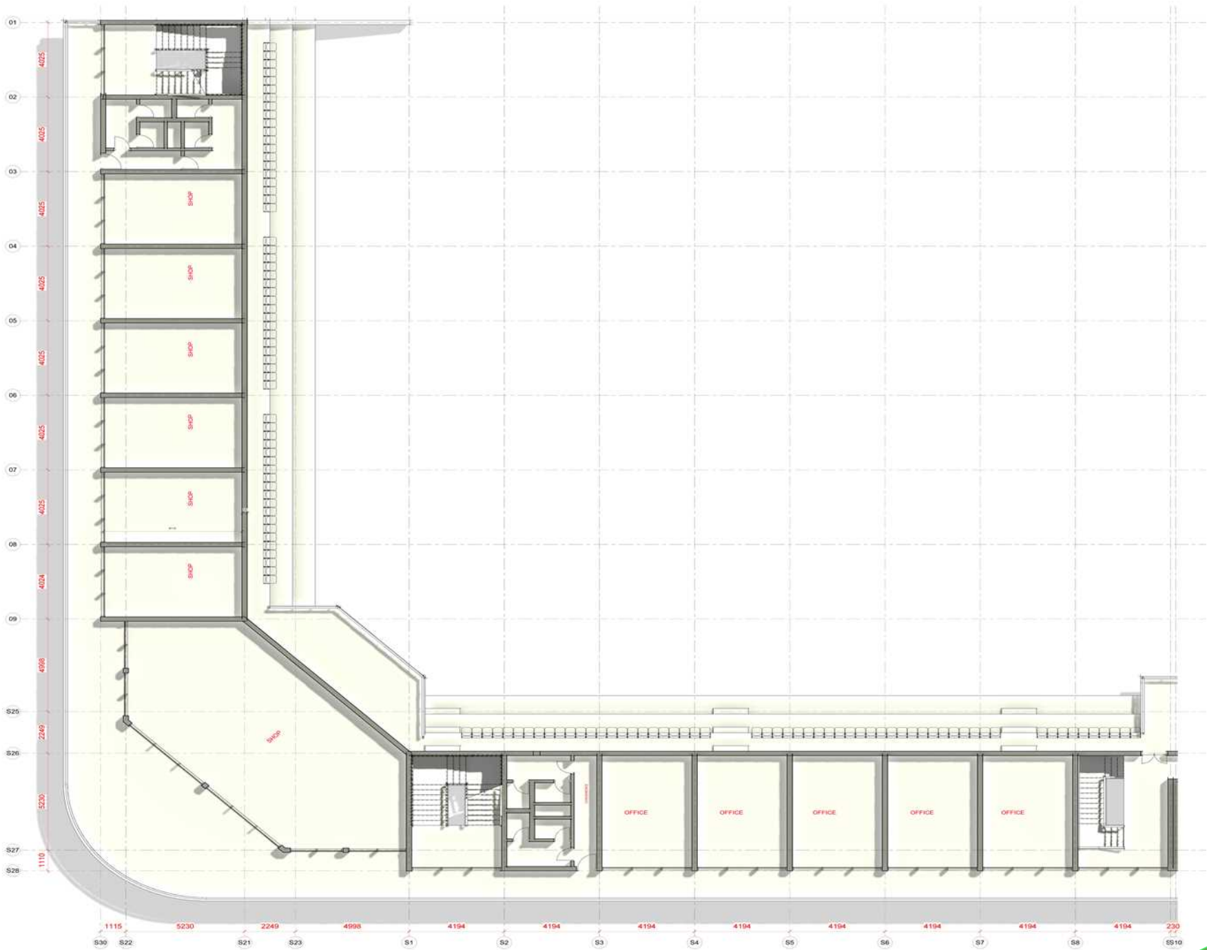
01- FIRST FLOOR PLAN
