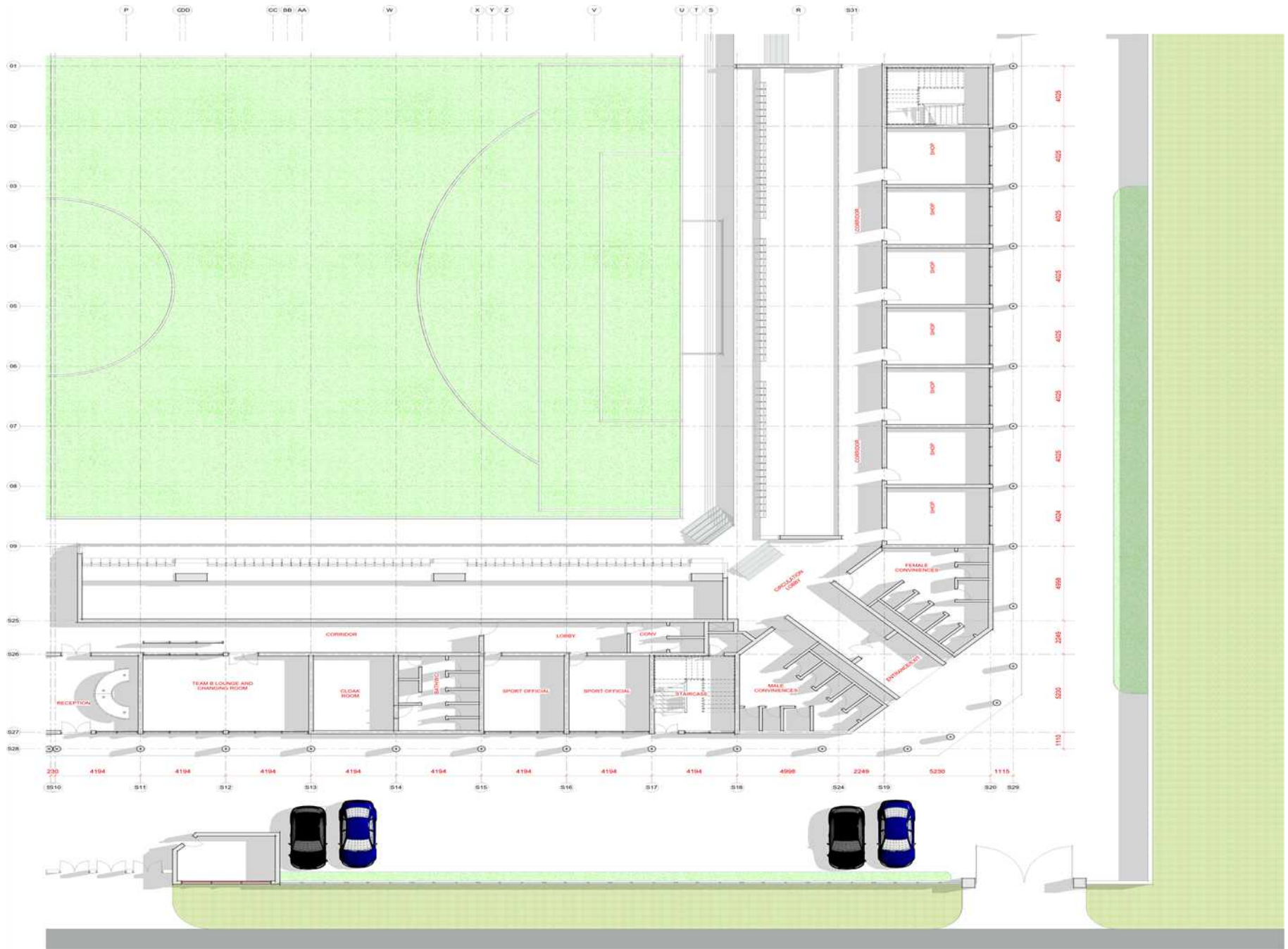
03b- GROUND FLOOR PLAN
